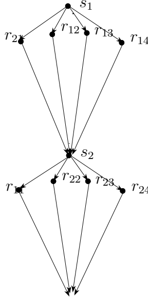
FIGURE 2. Auslander-Reiten-quiver: \Gamma^+(1 + 1 + 1 + 1)
