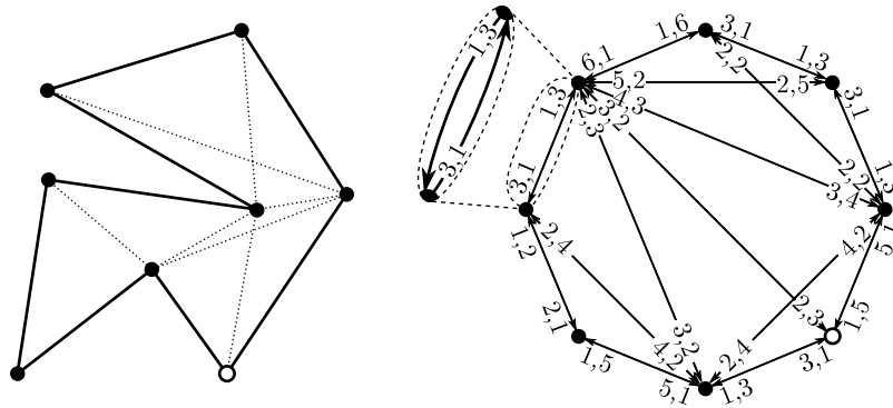
Fig. 19. An illustration of how the look-back capability can be encoded in the arc-labeling of G_{vis} from Fig. 13. The highlighted vertex is an ear and has a path with labels (1, 5), (4, 2) and a path with labels (3, 1), (2, 4), where 3 and 5 are the degrees of the vertex itself and its counter-clockwise neighbor, respectively.
