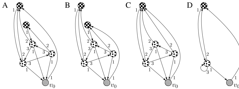
Fig. 15. Four graphs with local orientation that are indistinguishable to an agent initially located at vertex v_0 in terms of observations made by the agent along any walk. Vertices which appear indistinguishable (depicted with individual patterns of the nodes) to the agent can be merged in order to obtain smaller but still indistinguishable graphs.
