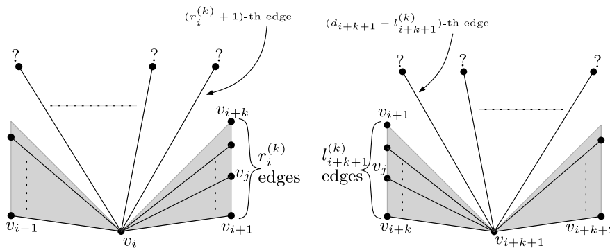
Fig. 8. Knowledge about the edges of v_i and v_{i+k+1} after step k of the algorithm. Left: the edges from v_i to vertices in \{v_{i+1}, \dots, v_{i+k}\} and in \{v_{i-1}, \dots, v_{i-k}\} have been identified. If v_i has r_i^{(k)} neighbors in \{v_{i+1}, \dots, v_{i+k}\} , then deciding whether v_i sees v_{i+k+1} is equivalent to deciding whether the (r_i^{(k)} + 1) -th edge of v_i leads to v_{i+k+1} . Right: If v_{i+k+1} has l_{i+k+1}^{(k)} neighbors in v_{i+1}, \dots, v_{i+k} , then deciding whether v_{i+k+1} sees v_i is equivalent to deciding whether the (d_{i+k+1} - l_{i+k+1}^{(k)}) -th edge of v_{i+k+1} leads to v_i .
