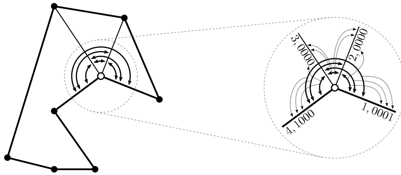
Fig. 21. Illustration of an angle-type sensor and how to encode it in the arc-labeling of G_{vis} .
