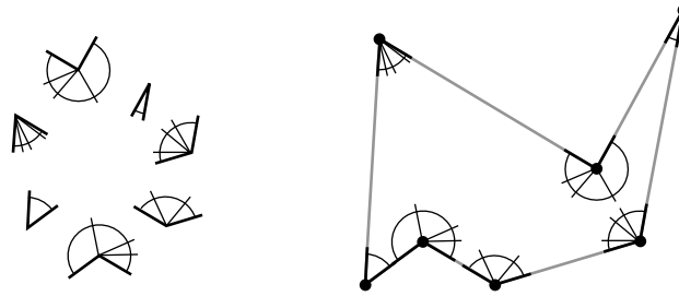
Fig. 5. Given the angle measurement for each vertex in counter-clockwise order (left), the goal is to find the unique polygon that fits these angle measurements (right).
