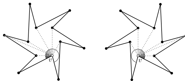
Fig. 10. Two polygons of different shape with the same set of angles at every vertex. The two polygons are mirror images of each other.
