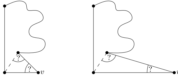
Fig. 12. Two polygons with angle measurements that differ in exactly two angles. This allows a single vertex v , which only sees its two neighbors along the boundary, to be at different positions in both polygons. Hence, the shape of a polygon cannot always be reconstructed if two or more angles are unknown.
