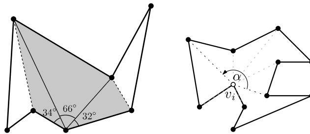
Fig. 4. Left: An angle measurement at a vertex yields the list of angles between adjacent edges of G_{vis} in counter-clockwise order, here (32^\circ, 66^\circ, 34^\circ) . Right: The angle between non-adjacent edges can easily be computed by summing the angles in between.
