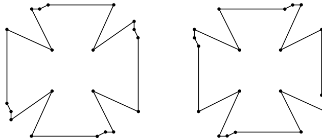
Fig. 24. Two polygons which appear indistinguishable to an agent with cvv and boundary-angle sensor that moves along the boundary. It can easily be verified that the same boundary angles and combinatorial visibility vectors appear in both polygons, and they appear in the same order along the boundary. Note that both polygons have the same number of vertices, thus knowledge of n does not help to distinguish them.
