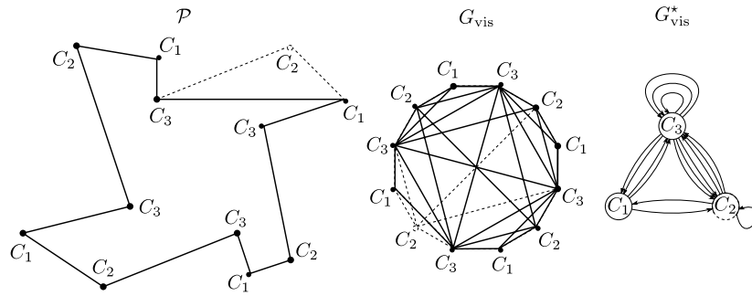
Fig. 16. A polygon \mathcal{P} together with its visibility graph G_{\text{vis}} and the minimum base graph G_{\text{vis}}^* . Here n = 12 and k = 3 , and every class contains 12/3 = 4 vertices. Cutting off a single vertex of \mathcal{P} (dashed parts) cannot easily be reflected in G_{\text{vis}}^* . In fact, in this example, the new base graph would need to have eleven vertices.
