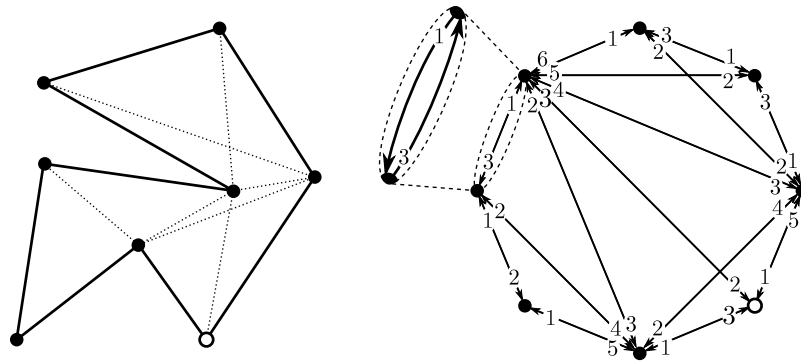
Fig. 13. A polygon with the corresponding directed and arc-labeled visibility graph. Every bidirected edge represents two arcs of opposite orientation.
