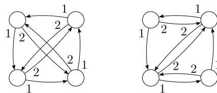
Fig. 14. Two graphs that cannot be distinguished by an agent with knowledge of n .
