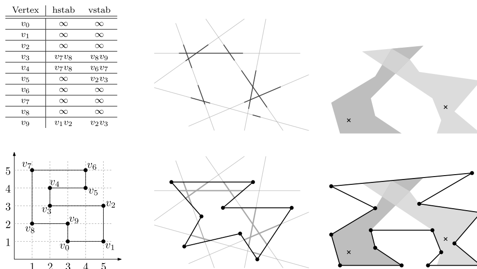
Fig. 25. Constructing consistent polygons from different kinds of data. From left to right: construction of orthogonal simple polygons from stabbing information; construction of polygons from line intersections; construction of simple polygons from visibility polygons of certain points in the interior.
