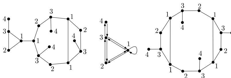
Fig. 27. Two non-isomorphic graphs G (left), H (right) that are indistinguishable together with their minimum base graph B (center). The numbers on the nodes represent the equivalence classes with respect to symmetry. Edge labels are omitted to not clutter the figure.
