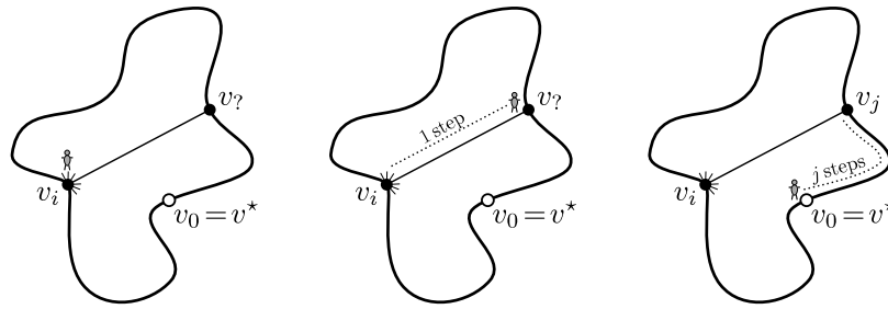
Fig. 2. If the agent can distinguish some vertex v^* (in our example v^* = v_0 ), it can easily determine where edges lead: starting at a vertex v_i , the agent can identify the target of an edge by moving along this edge and then along the boundary until it encounters v^* , counting the number of moves it makes.
