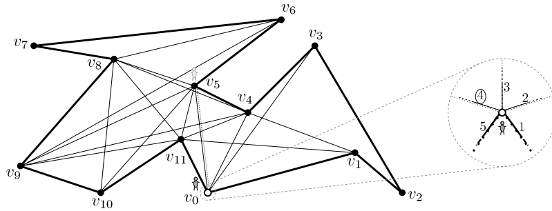
Fig. 18. The perception of the agent with look-back capability after its move from v_5 to v_0 . The agent can distinguish the arc leading back to v_5 , i.e., it knows this index “4” of this arc in the local ordering.
