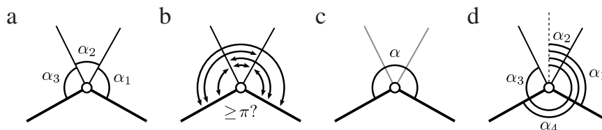
Fig. 22. Local perception with different kinds of angle sensors. From left to right: standard angle sensor, angle type sensor, boundary angle sensor, direction sensor combined with angle sensor.
