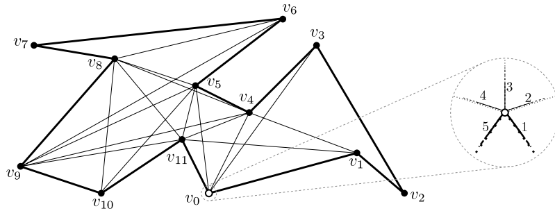
Fig. 1. Left: A simple polygon with embedded visibility graph. Right: The polygon as perceived locally by an agent located at v_0 . All that the agent can observe is an order of the edges incident to its location. Except for the two boundary edges, the agent does not know to which vertex, or in which direction, each edge leads.
