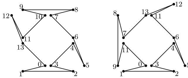
Fig. 11. Two different polygons with the same set of angle measurements. Every angle measurement of a vertex in the left polygon also appears as the angle measurement of a vertex in the right polygon. The order in which these measurements occur along the boundary is different however.
