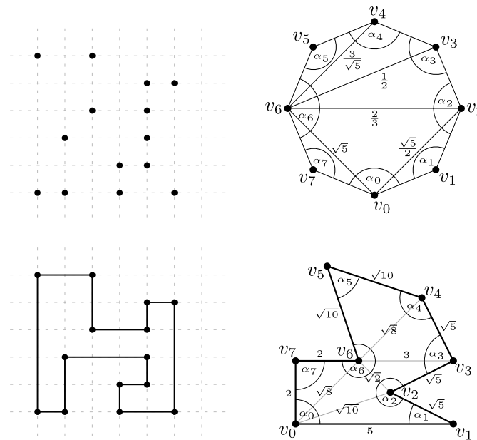
Fig. 26. Reconstructing a polygon from different kinds of data. Left: reconstruction of an orthogonal simple polygon from the coordinates of its vertices. Right: reconstruction of a simple polygon from the triangulation of its visibility graph with cross-ratios and boundary angles. The top figure shows the underlying triangulation of the polygon, where each edge is labeled by the cross-ratio of the corresponding quadrilateral. The bottom picture shows the underlying triangulation of the polygon, where each edge is labeled by its length.
