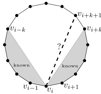
Fig. 7. State of the reconstruction of G_{\text{vis}} after step k of the algorithm. For every vertex v_i , the neighbors of v_i in \{v_{i+1}, \dots, v_k\} have already been identified. Hence, the subgraphs of G_{\text{vis}} depicted by the shaded areas have been fully reconstructed. In the next step, the algorithm has to decide whether v_i sees v_{i+k+1} , and thus whether \{v_i, v_{i+k+1}\} is an edge of G_{\text{vis}} .
