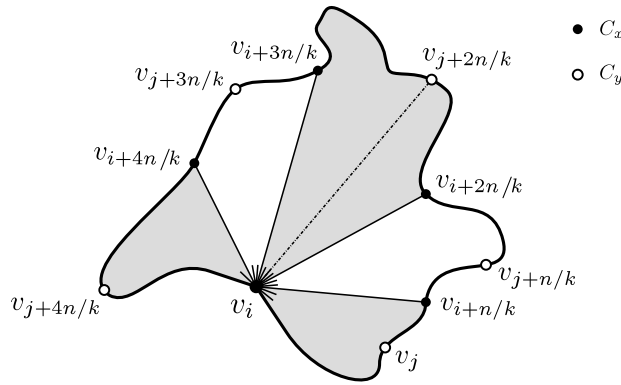
Fig. 20. A vertex v_i in a class C_x that forms a clique in G_{vis} has an arc to every other vertex of C_x . These arcs divide \mathcal{P} into sectors (depicted as the alternating shaded and white areas), such that each class appears exactly once in every sector. From G_{vis}^* , the agent knows to which class C_y an arc leads, and it also knows the sector into which the arc falls. This is enough to uniquely identify the exact target of the arc. Here, k = 5 and j = i + ((y - x) \bmod k) .
