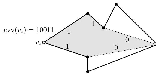
Fig. 23. The combinatorial visibility vector of a vertex v_i encodes which vertices visible to v_i are neighbors along the boundary. The shaded area is the subpolygon induced by the visible vertices of v_i .
