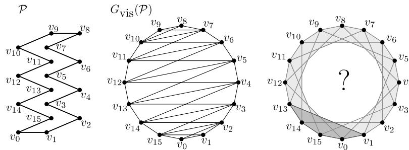
Fig. 6. Progress of the reconstruction of a polygon \mathcal{P} after step k = 4 . From left to right: the polygon \mathcal{P} , its visibility graph G_{\text{vis}} of \mathcal{P} , and the subgraphs of G_{\text{vis}} that have fully been reconstructed after k = 4 steps (schematically depicted as shaded areas – no edges of the visibility graph are depicted). All subgraphs of G_{\text{vis}} induced by k + 1 = 5 consecutive vertices (shaded areas) are already fully reconstructed. Edges between vertices that are more than k steps apart along the boundary have not been reconstructed yet.
