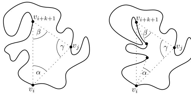
Fig. 9. Schematic illustration of the induction step of the reconstruction of G_{vis} . Left: If v_i sees v_{i+k+1} , there has to be a vertex v_j in \{v_{i+1}, \dots, v_{i+k}\} which sees both v_i and v_{i+k+1} , and v_i, v_j, v_{i+k+1} form a triangle in G_{vis} . Right: If v_i does not see v_{i+k+1} , and v_j sees v_i and v_{i+k+1} at an angle \gamma < \pi , the boundary of \mathcal{P} between v_{i+k+1} and v_i (in this order) has to block the line of sight between v_i and v_{i+k+1} .
