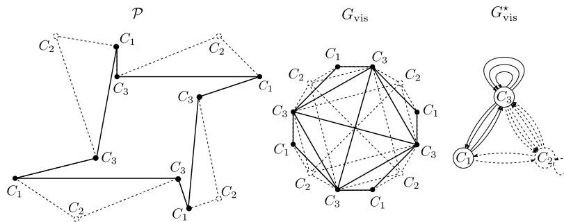
Fig. 17. Cutting off an entire class of ears can easily be done in G_{\text{vis}}^* by removing the corresponding vertex entirely.
