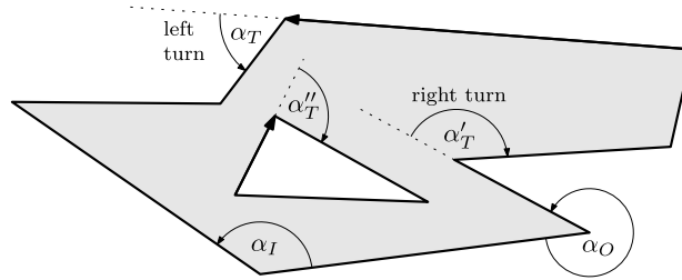
Fig. 5. A polygon with inner angle \alpha_I , outer angle \alpha_O and three turn angles \alpha_T > 0 , \alpha'_T < 0 , and \alpha''_T < 0 . Observe that \alpha_T and \alpha'_T are the turn angles in counterclockwise direction, whereas \alpha''_T is the turn angle in clockwise direction.
