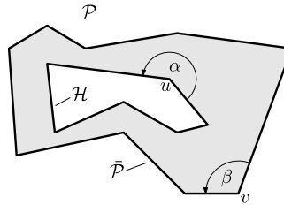
Fig. 6. Inner angles of polygon \mathcal{P} : \alpha is the inner angle of the polygon at vertex of u \in \mathcal{H} and \beta is the inner angle of the polygon at vertex v \in \bar{\mathcal{P}} . Observe that when \mathcal{H} is considered as a simple polygon, then \alpha is its outer angle.
