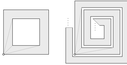
Fig. 4. The left polygon is a square with a square hole. The right polygon is a “spiral” – a polygon without a hole. A robot observes exactly the same in both polygons, regardless of its movements, unless it reaches the end of the spiral.
