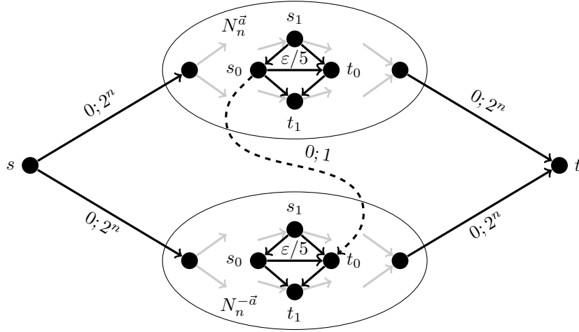
Figure 2: Illustration of network G_{\text{ssp}}^{\vec{a}} . The subnetworks N_n^{\vec{a}} and N_n^{-\vec{a}} are advanced independently by the Successive Shortest Path Algorithm without using arc e , unless the PARTITION instance \vec{a} has a solution.
