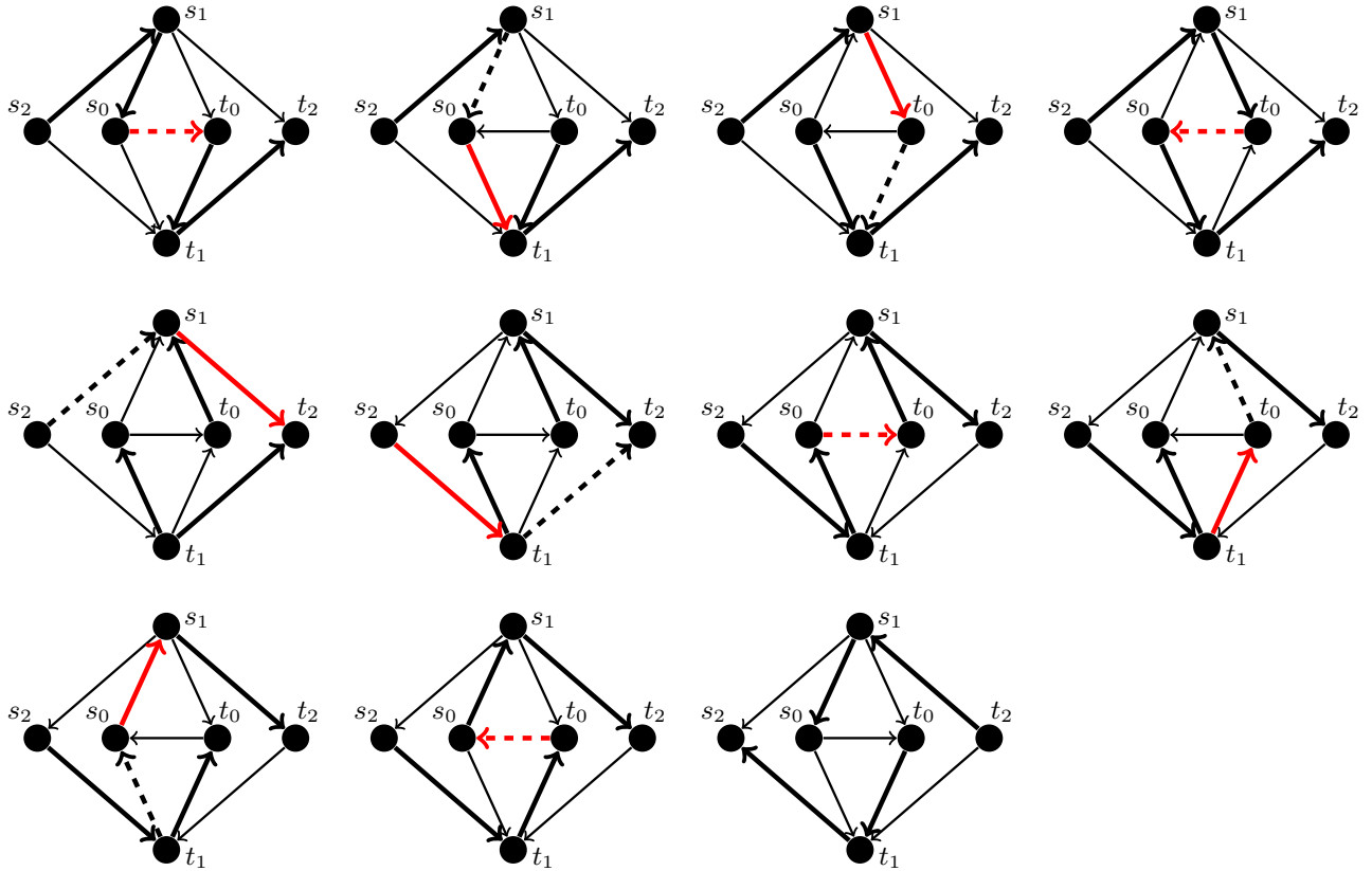
Figure 4: Illustration of the iterations performed by the Network Simplex Algorithm on the counting gadget S_2^{\vec{a},r} for r < 1/2 . The external tree-path from t_2 to s_2 is not shown. Bold arcs are in the basis before each iteration, the red arc enters the basis and the dashed arc exits the basis. Arcs are oriented in the direction in which they are used next. Note that after 2x_2 = 3 \cdot 2^2 - 2 = 10 iterations the configuration is the same as in the beginning if we switch the roles of s_2 and t_2 .
