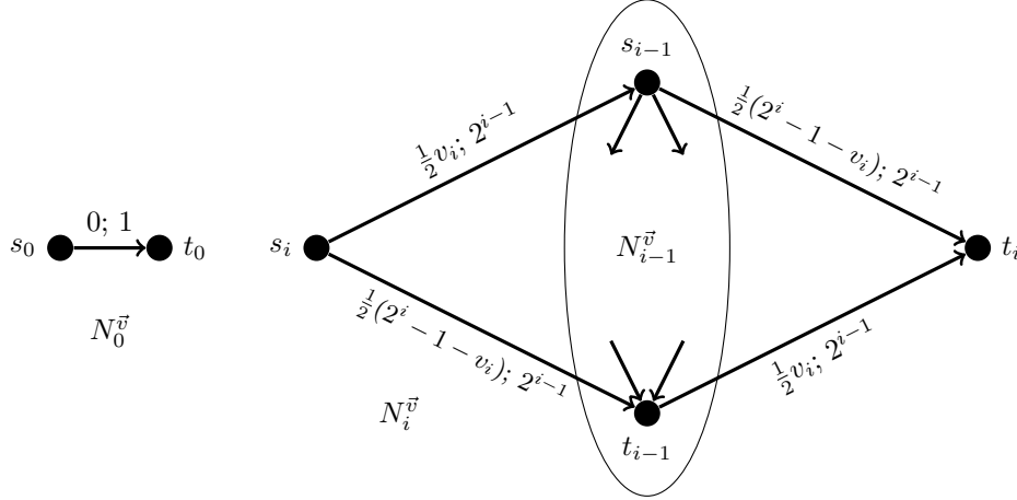
Figure 1: Recursive definition of the counting gadget N_i^{\vec{v}} for the Successive Shortest Path Algorithm and \vec{v} \in \{\vec{a}, -\vec{a}\} . Arcs are labeled by their cost and capacity in this order. The cost of the shortest s_i - t_i -path in iteration j = 0, \dots, 2^i - 1 is j + \vec{v}_i^{[j]} .
