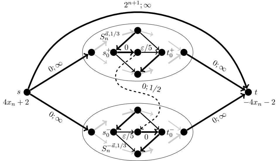
Figure 5: Illustration of network G_{ns}^{\bar{a}} . The subnetworks S_n^{\bar{a}, 1/3} and S_n^{-\bar{a}, 1/3} are advanced independently by the Network Simplex Algorithm without using the dashed arc e , unless the PARTITION instance \bar{a} has a solution. Bold arcs are in the initial basis and carry a flow of at least 1 throughout the execution of the algorithm.
