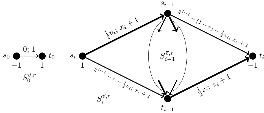
Figure 3: Recursive definition of the counting gadget S_i^{\vec{v},r} for the Network Simplex Algorithm, \vec{v} \in \{\vec{a}, -\vec{a}\} , and a parameter r \in (2A, 1 - 2A) , r \neq 1/2 . The capacities of the arcs of S_i^{\vec{a},r} \setminus S_{i-1}^{\vec{a},r} are x_i + 1 = 3 \cdot 2^{i-1} . If we guarantee that there always exists a tree-path from t_i to s_i with sufficiently negative cost outside of the gadget, the cost of iteration 3k , k = 0, \dots, 2^i - 1 , within the gadget is k + \vec{v}_i^{\lfloor k \rfloor} . Bold arcs are in the initial basis and carry a flow of at least 1 throughout the execution.
