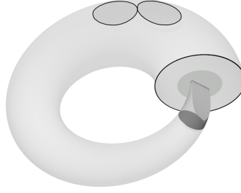
FIGURE 1. A geometric non-Lipschitzian setting which fulfills our assumptions, if the grey apex and the three shaded circles carry the Dirichlet condition
