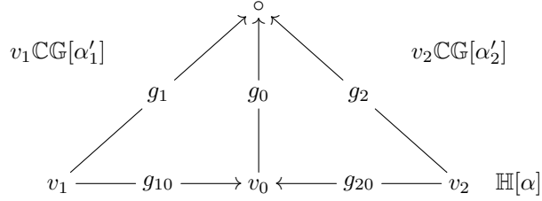
Figure 2: Pattern for identifications in \text{CE}(\mathbb{H}[\alpha], \mathbb{G}, \alpha) , see (†) in Definition 7.1: for i = 1, 2 , g_{i0} = [w_{i0}]_{\mathbb{G}} links v_0 to v_i in their \alpha'_i -component of \mathbb{H} .
