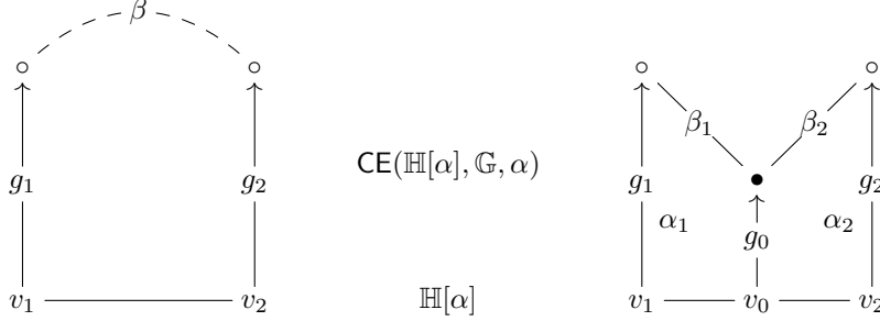
Figure 4: Bridge-freeness.
