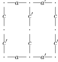
Figure 1: Amalgamated cycles as in Example 2.13
