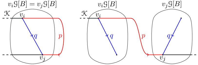
FIGURE 4. Part of \mathcal{K} \cup \bigcup_{t=1}^k v_t\mathcal{G}[B] \subseteq \mathcal{G}[A] and of \text{CE}(G, \mathcal{K}; B)
